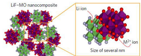
Molecular structure of LFM nanocomposite
