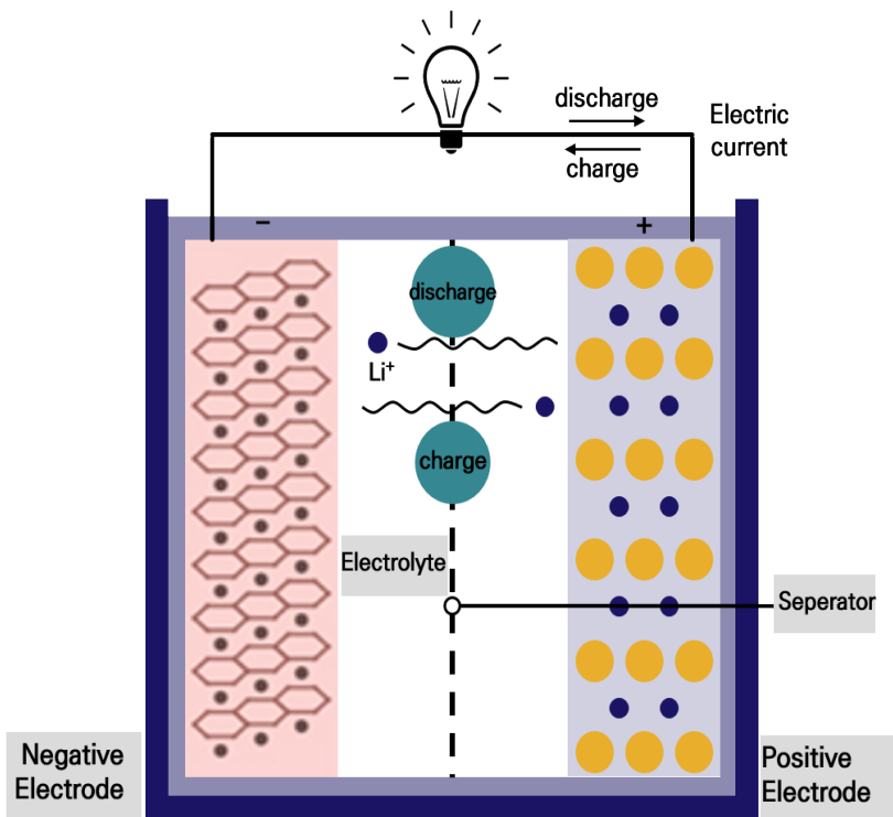
Battery Structure
